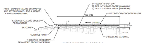
HIKE & BIKE TRAIL (LONGITUDINAL SECTION) TYPICAL
